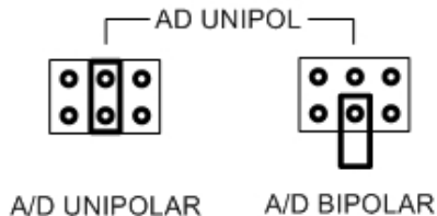
Figure 25: A/D Unipolar/Bipolar Selection
