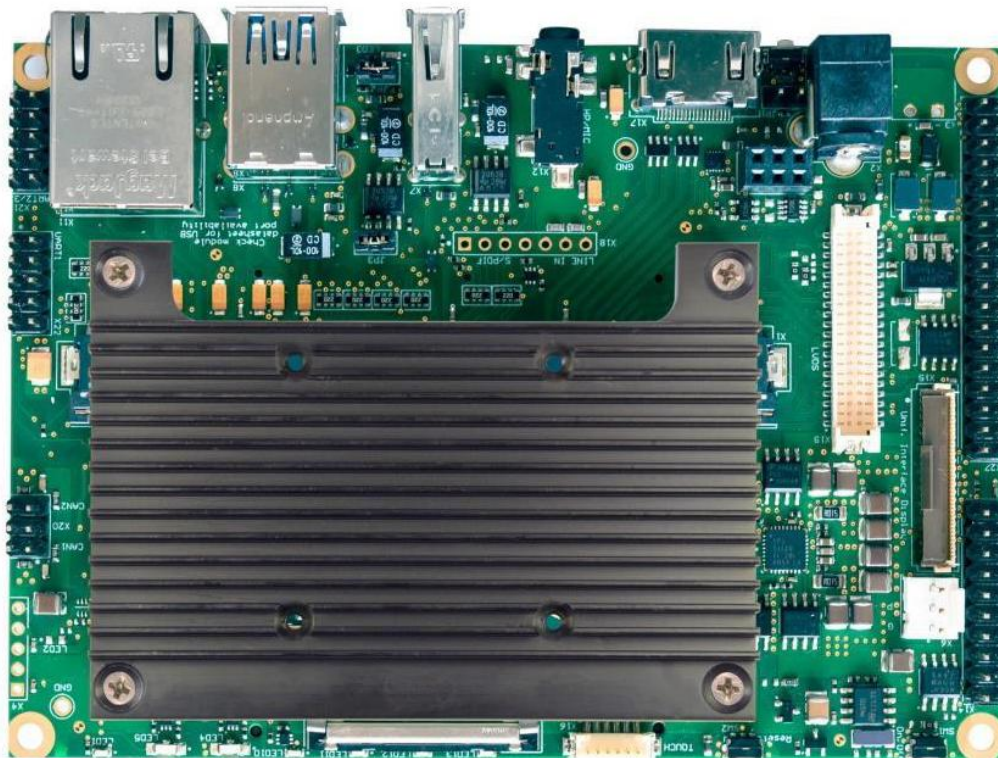
Figure 24 Affix heatsink with the system using M3 sized screws
