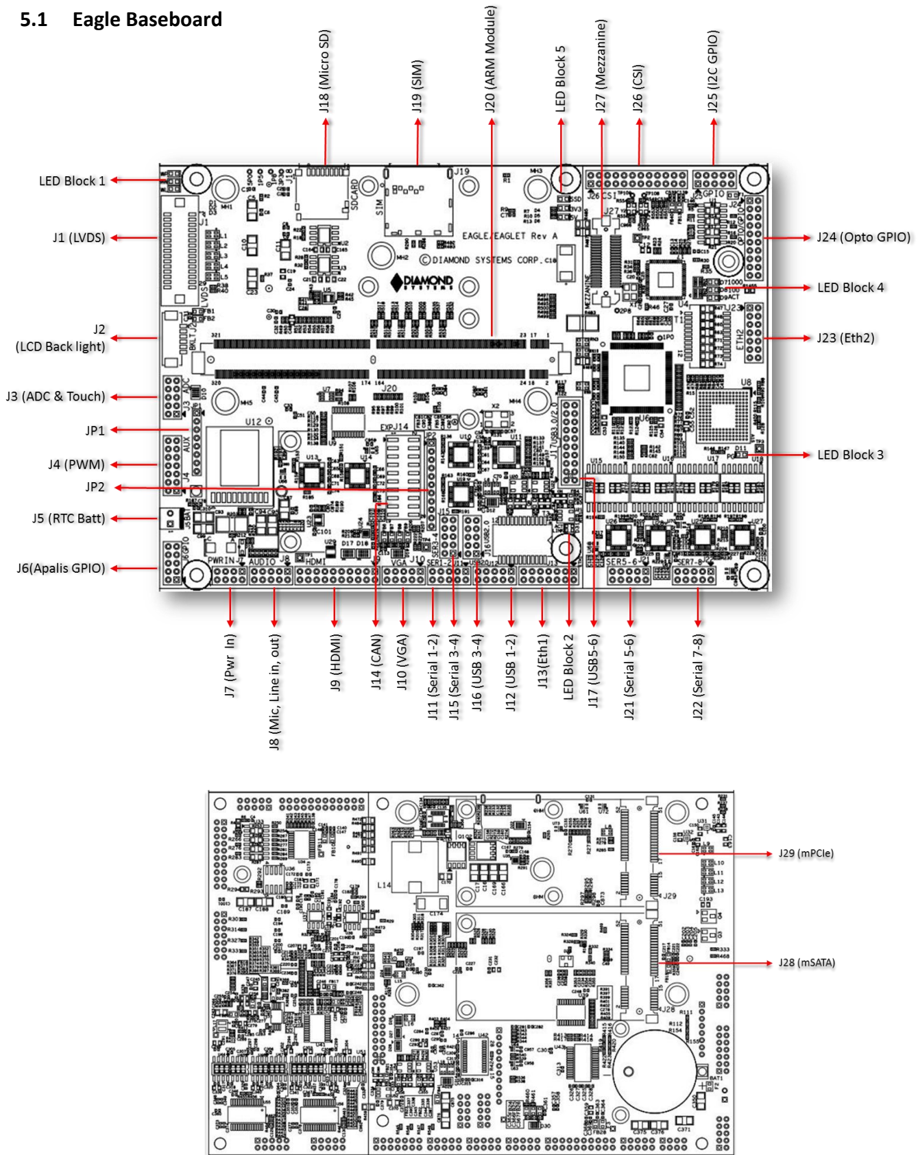
Figure 8 Board Layout, Top view and bottom view
