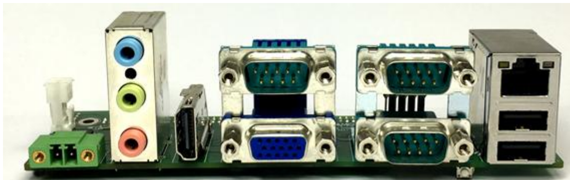
Figure 18 Panel IO board Front View
