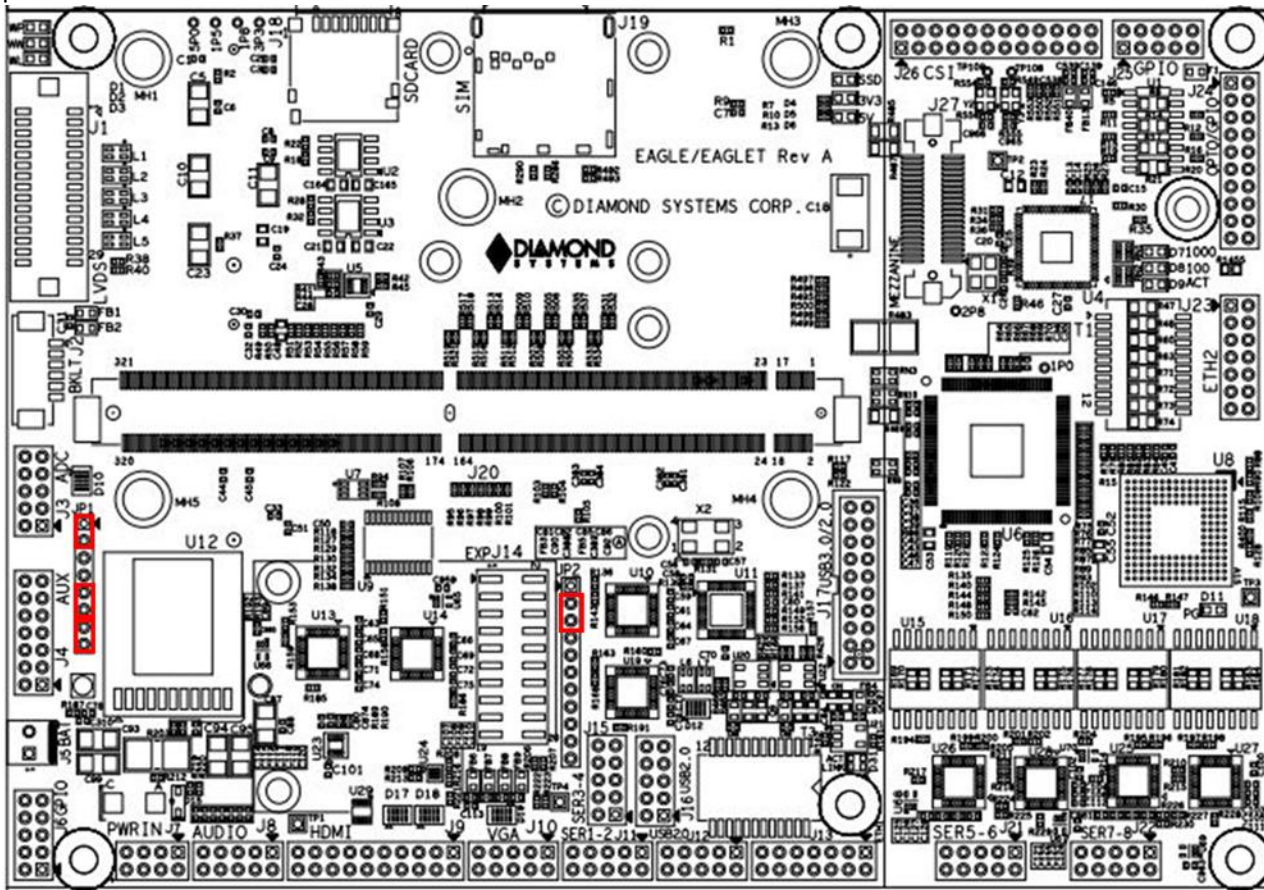
Figure 10 Default Jumper locations
