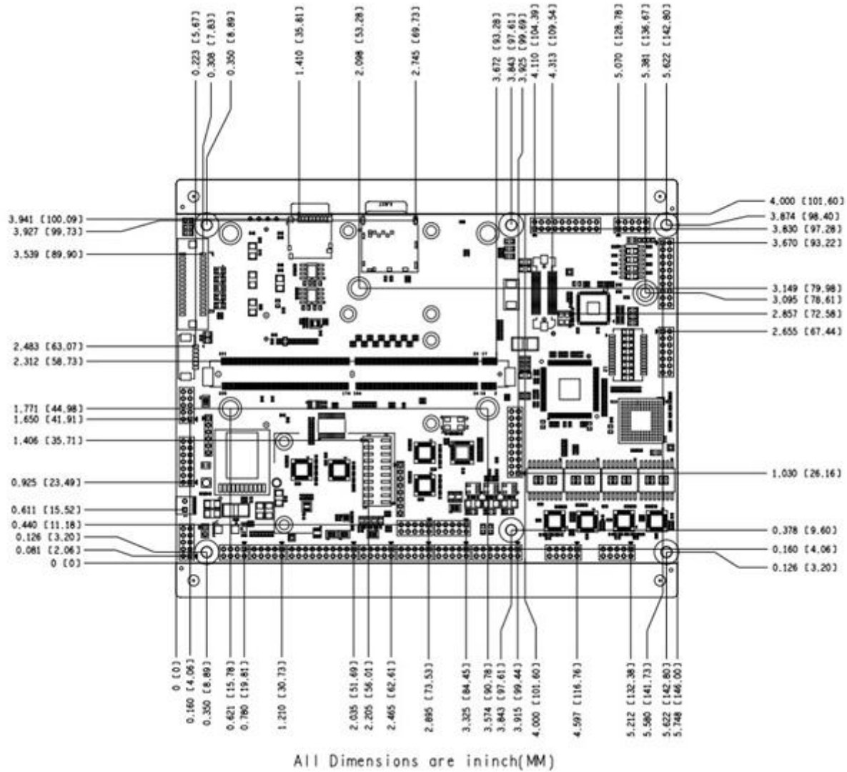
Figure 7 Eagle Baseboard Mechanical drawing
