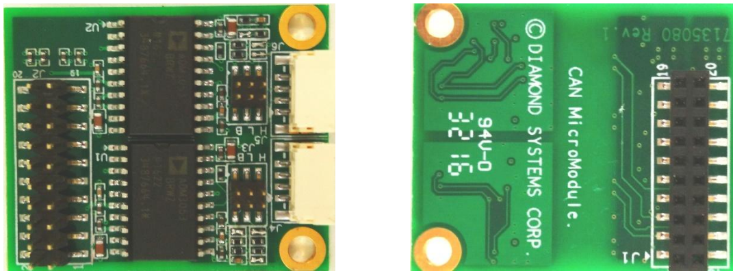
Figure 20 DS-MPE-CAN2L Front view (on left), rear view (on right)
