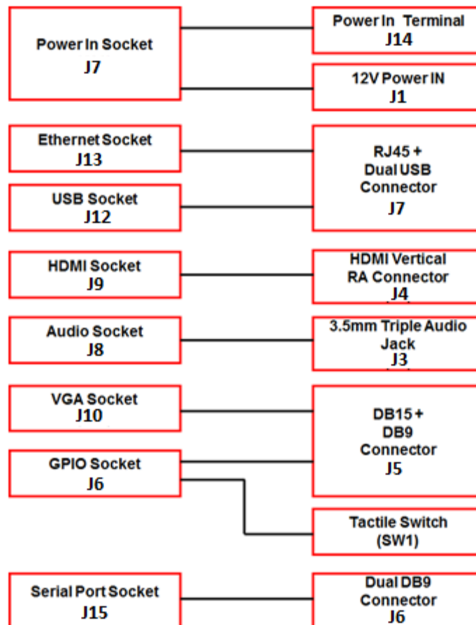
Figure 19 Panel IO to Eagle Connection
