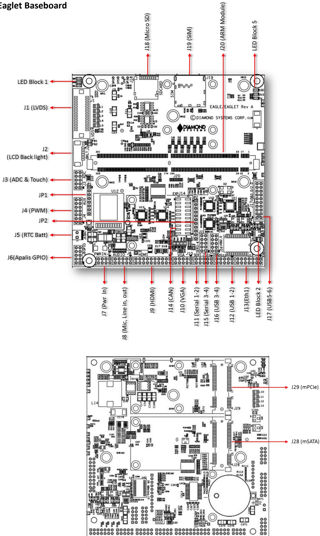
Figure 9 Eaglet board layout, Top and bottom view
