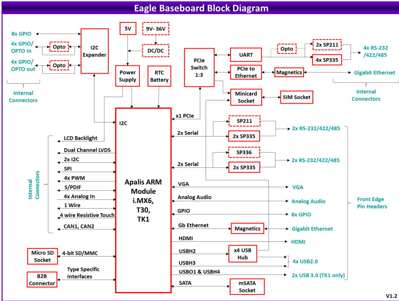
Figure 2 Functional Block Diagram of Eagle
