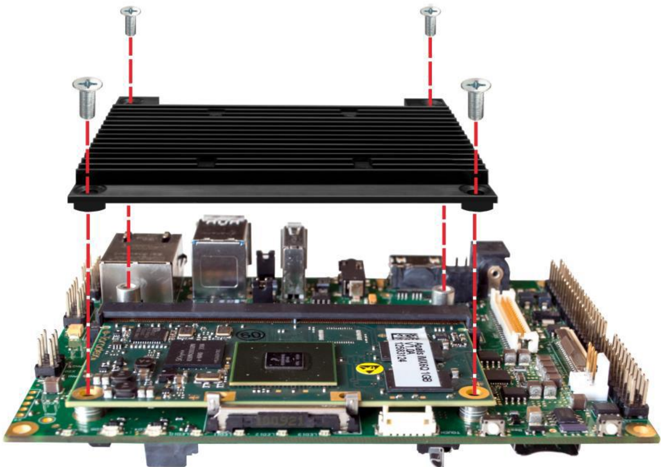
Figure 21 Apalis Heatsink Assembly
