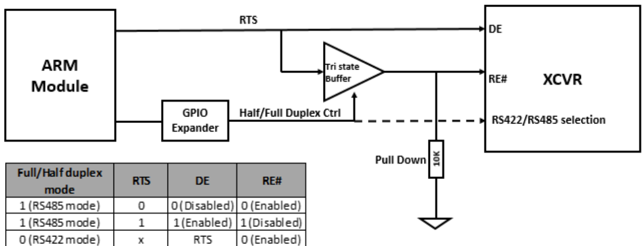
Figure 14 RS-485 direction control hardware implementation
