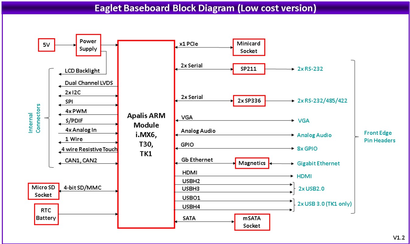
Figure 1 Functional Block Diagram of Eaglet
