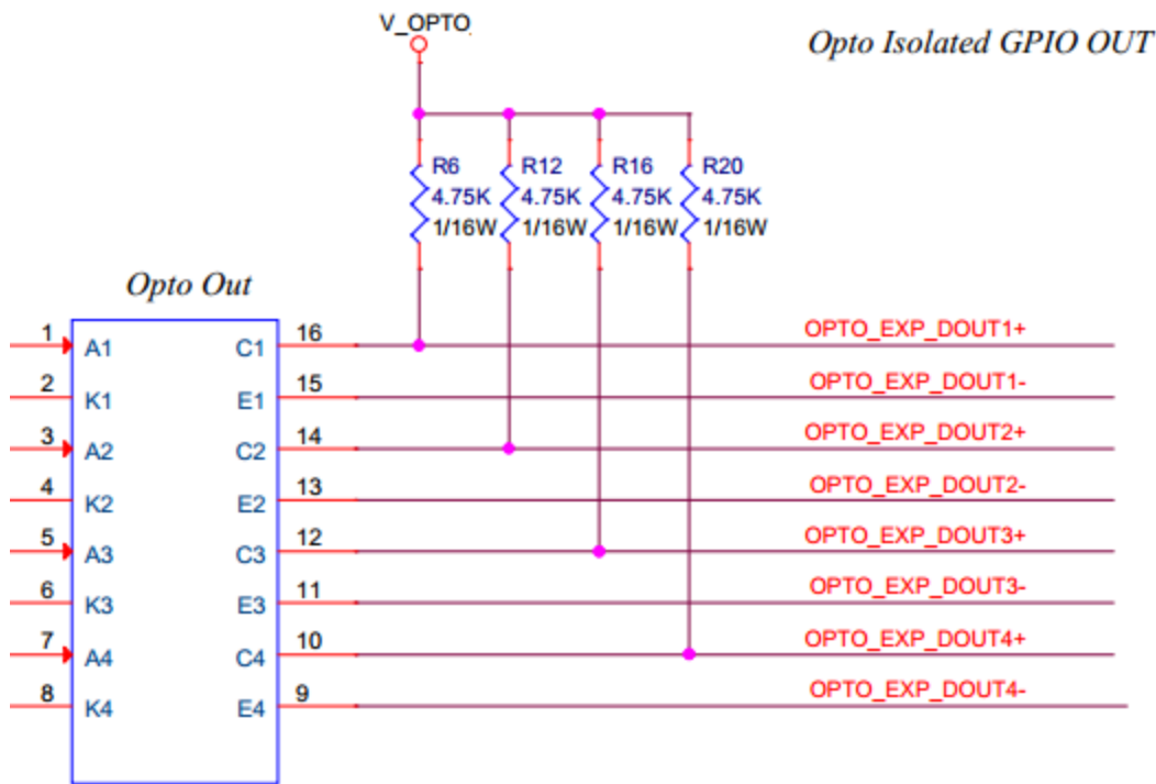
Figure 16 Opto isolated outputs hardware implementation
