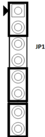
Figure 11 Jumper Block JP1
