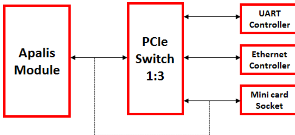
PCIe lane is connected directly to Mini PCIe slot in Low cost Eaglet baseboard
