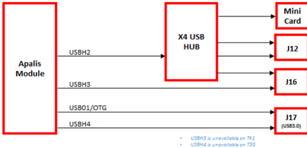
Figure 3 USB Signal connection for Eagle baseboard
